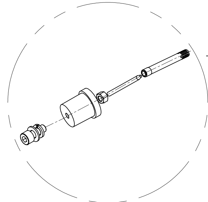
View - A Details Anchor Bolt assembly Enlarged View
